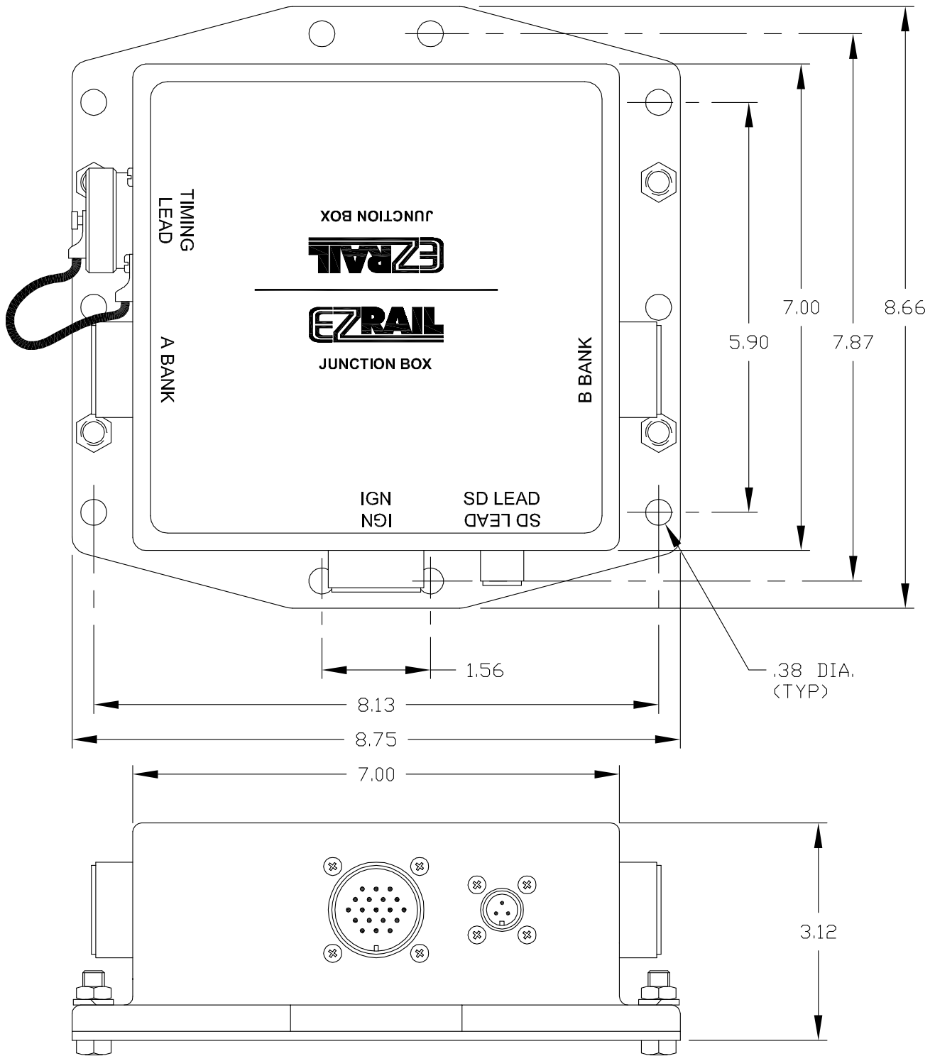
FIGURE 2 – DIMENSIONS: J-BOX
